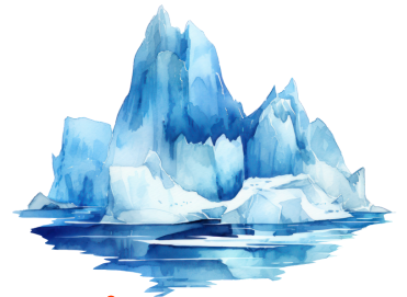
g lacier
